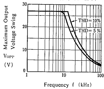
Maximum Output Voltage Swing vs. Frequency ( V^+/V^- = \pm 15V , T_a = 25^\circ C )
